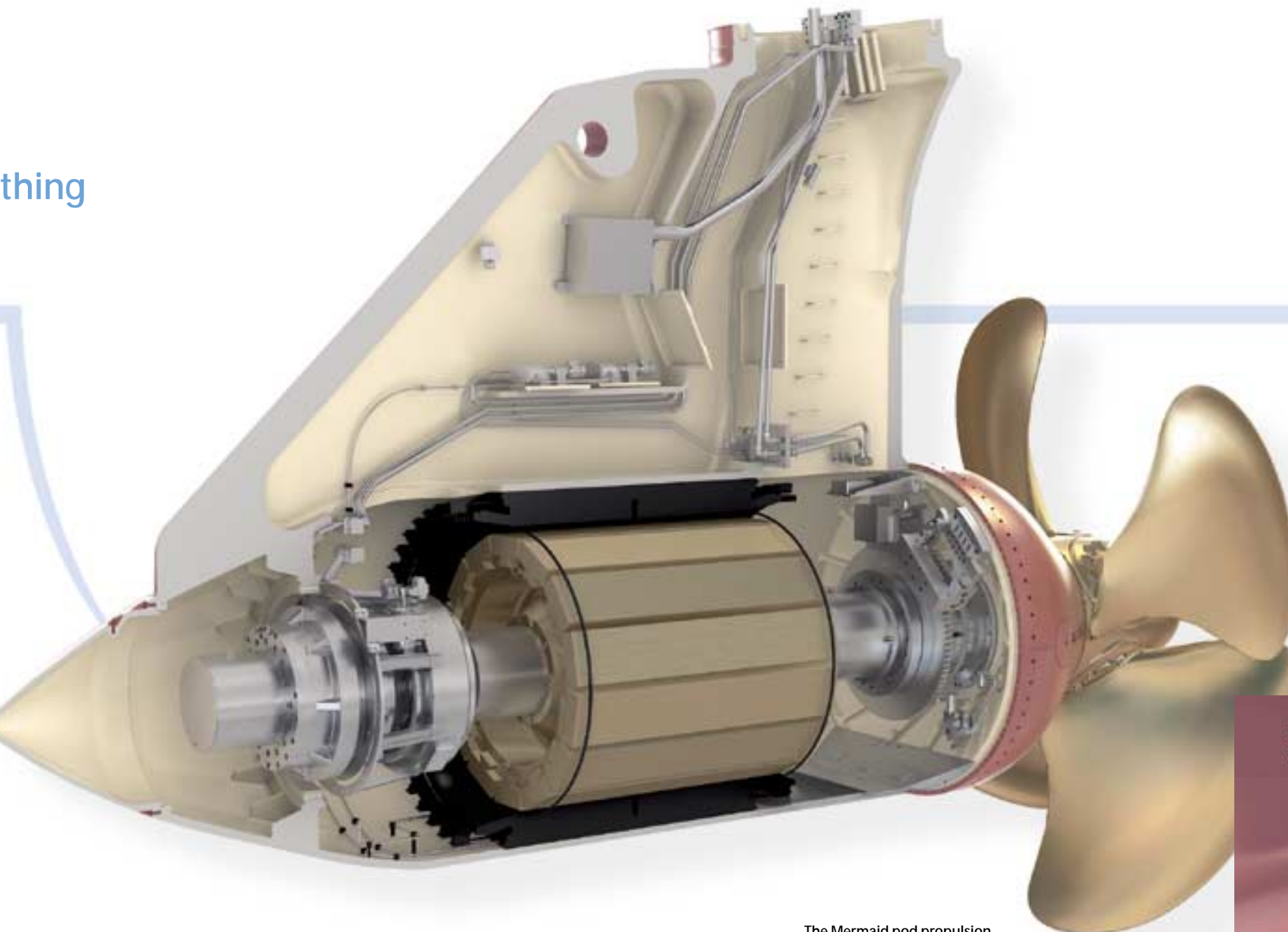
The Mermaid pod propulsion system is available from 5-25 MW.
