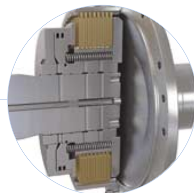
The gearbox is equipped with a mechanical driven servo oil pump, ensuring continuous oil supply also when the main clutch is disengaged.
