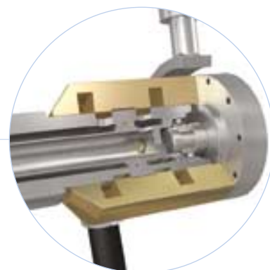
The oil distribution valve is of simple and reliable design. It floats on the oil distribution shaft.
