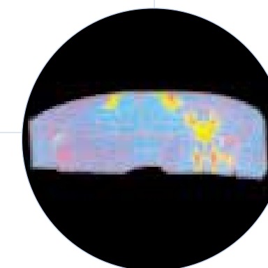
Diagram showing stress concentrations in blade attachment area.
